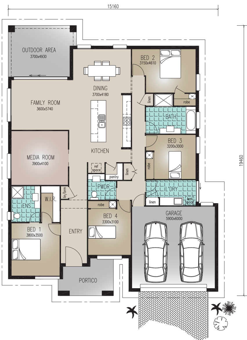
Perspective & Floor Plan are artists impressions only
